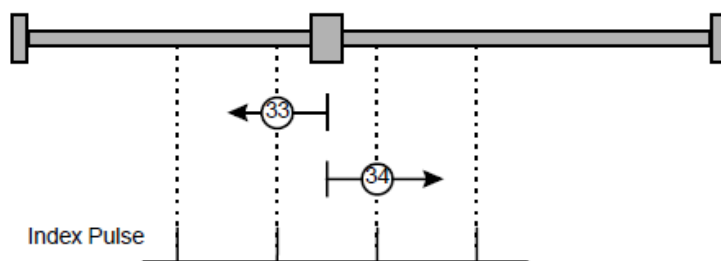
图 4-1 Homing Method 33&34
